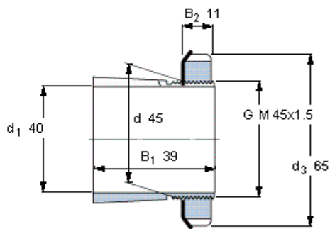
External taper of 1:12
