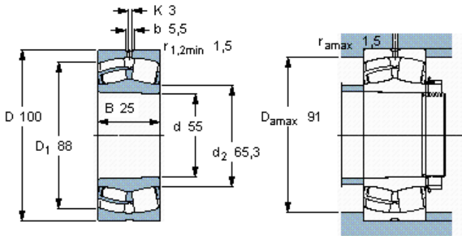
Tapered bore, taper 1: 12
